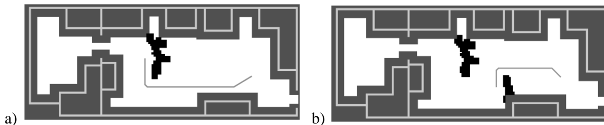
Figure 96. a) An avoidance maneuver was generated by the path planner to clear the row of cylinders shown in Figure 95a. b) Revised path from robot's new position to accommodate the discovery of the cart shown earlier in Figure 95a (adapted from Everett, Gilbreath, & Tran, 1990).
