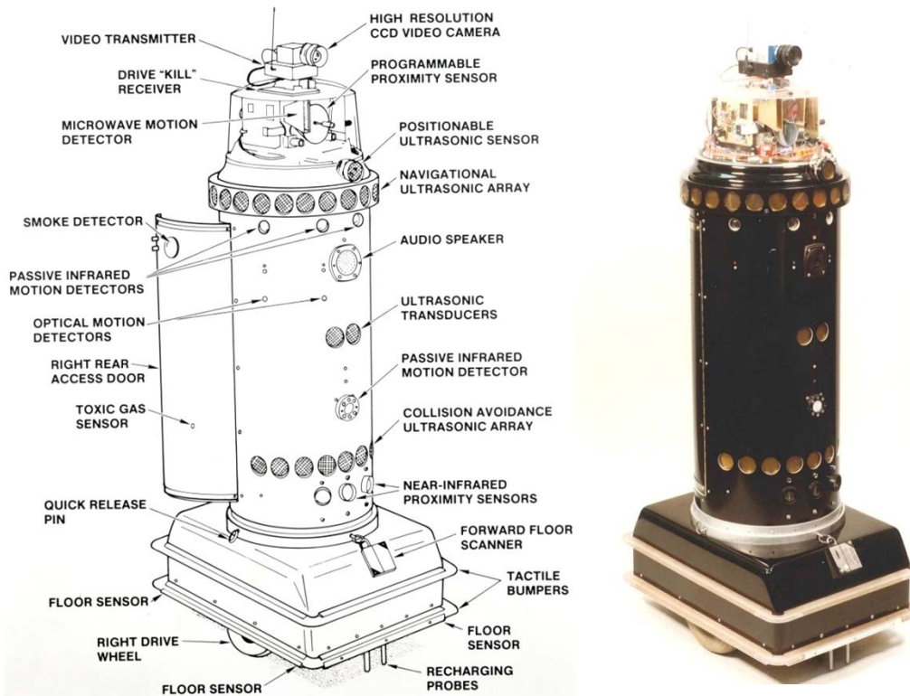
Figure 98. ROBERT II was equipped with an array of environmental, intrusion detection, and navigation sensors. The upgraded Polaroid sonar system featured 36 electrostatic transducers (versus the original six) in two separate arrays. The upper body easily detached from the mobility base upon removal of four quick-release pins.
