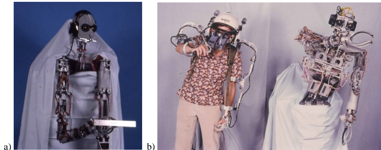
Figure 87. a) Early “Green Man” prototype, circa 1983. b) Developed by Code 53 at the NOSC Hawaii Laboratory, this 1985 version (right) mimics the head and torso movements of operator Dave Smith (left). The stereo cameras on this configuration were integrated by avionics contractor Teledyne (Umeda, 2015).
